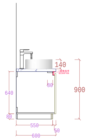
SECTION VIEW
