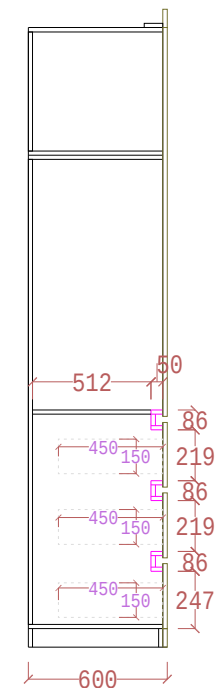
SECTION VIEW
