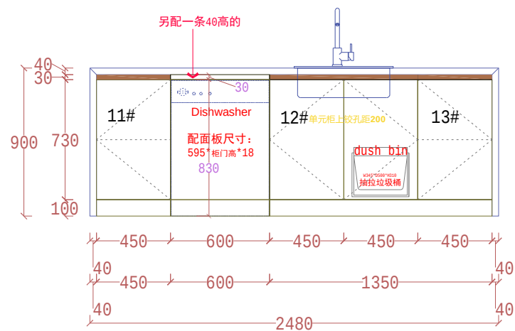
ELEVATION F
