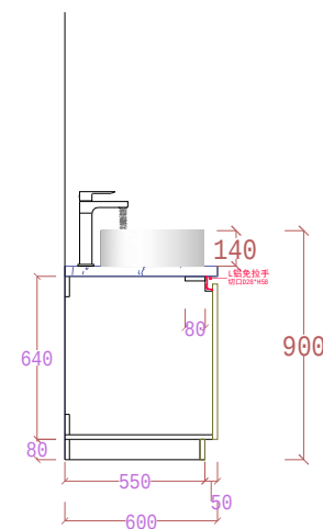
SECTION VIEW
