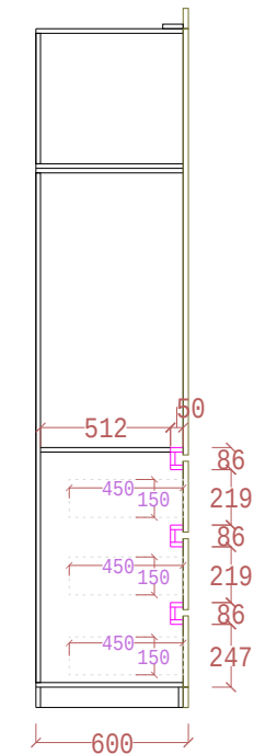
SECTION VIEW
