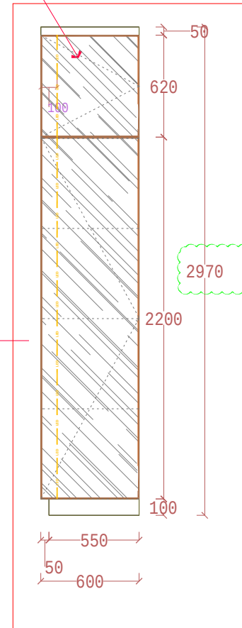
SIDE VIEW
