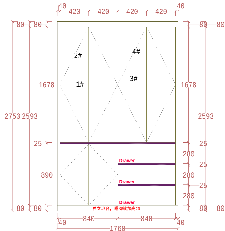
OUTSIDE VIEW
