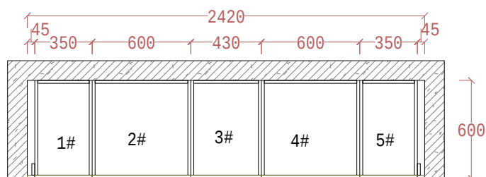
PLAN VIEW floor
