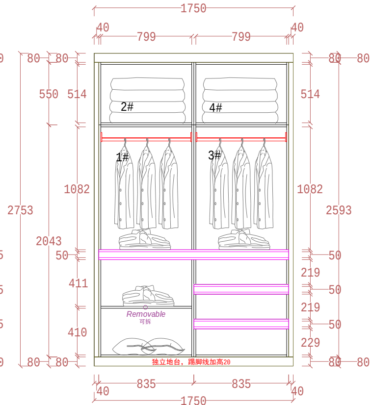
INNER VIEW
