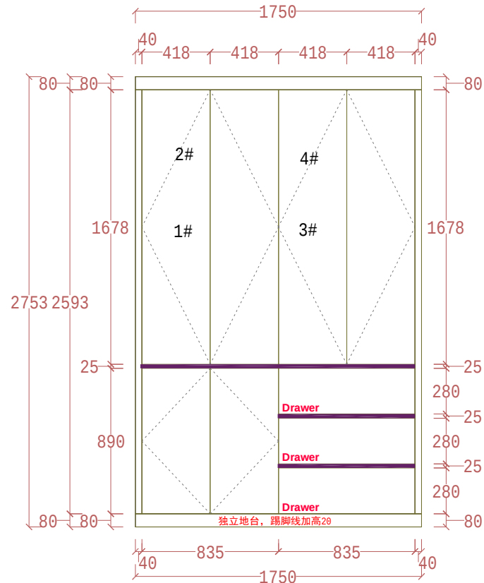
OUTSIDE VIEW
