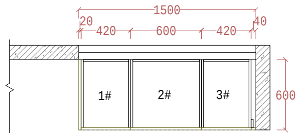
PLAN VIEW floor
